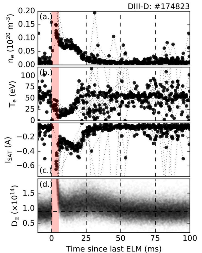
Fig. 3. Plasma behavior in the outer divertor as a function of ELM-period. Density (a), temperature (b) and saturation current (c) are all read from a Langmuir probe near the outer strikepoint. The D_\alpha measurement in (d) is taken from a filterscope aimed at the strikepoint location. The ELM crash is shaded in red. (For interpretation of the references to color in this figure legend, the reader is referred to the web version of this article.)
