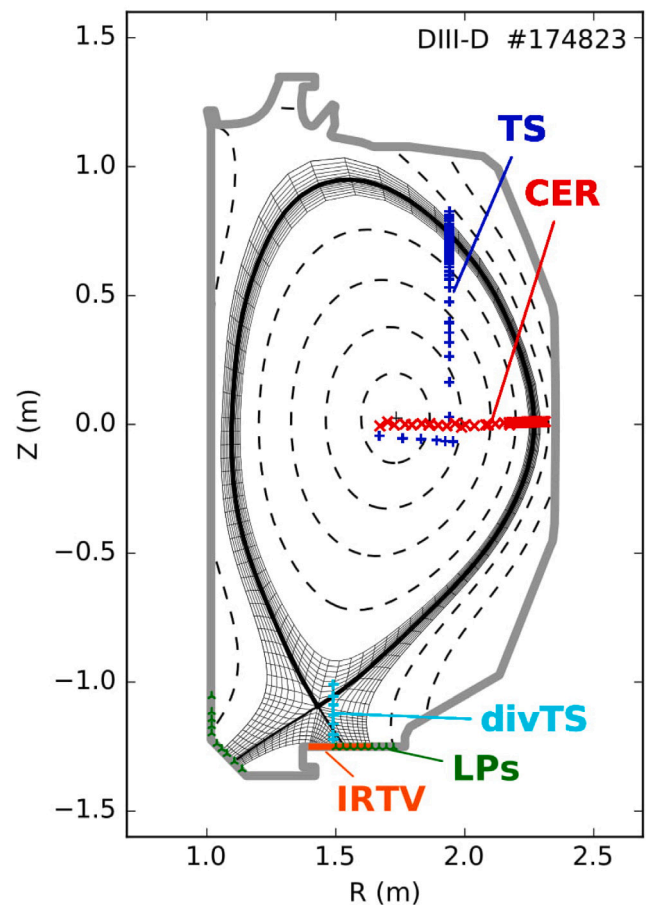
Fig. 1. An overview of the considered diagnostics is overlaid on top of an example equilibrium and UEDGE grid. TS (blue) and CER (red) are used to construct core profiles, whereas divertor TS (cyan), IRTV (orange) and Langmuir Probes (green) are used for divertor analysis. D_\alpha filterscopes aimed at the top and bottom divertor areas are not shown. (For interpretation of the references to color in this figure legend, the reader is referred to the web version of this article.)
