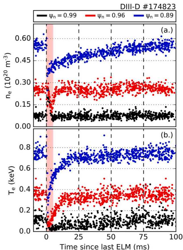
Fig. 4. Electron density (a) and temperature (b) measurements as a function of time since the last ELM. Little change is observed at the separatrix (black), data in the middle of the pedestal (red) experiences a rapid rise after the ELM and data at the top of the pedestal (blue) rises on a slower timescale until the onset of the next ELM. (For interpretation of the references to color in this figure legend, the reader is referred to the web version of this article.)
