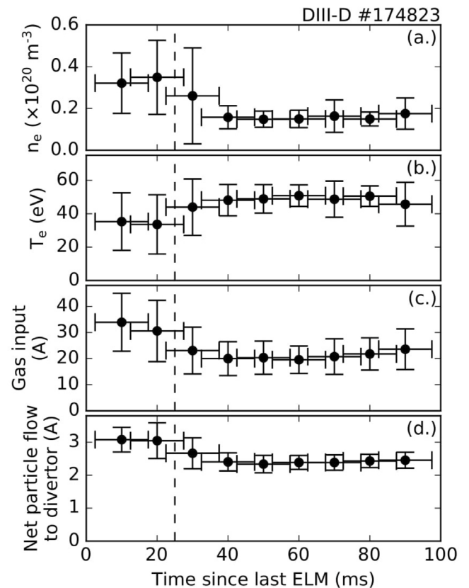
Fig. 7. ELM-synced averages of divertor parameters from \sim 125 converged UEDGE simulations. (a) The peak n_e along the outer divertor shows the same behavior as the LP traces in Fig. 3, with elevated divertor densities before \sim 25 ms. Also shown are the (b) the divertor T_e , (c) the external gas source determined by the code and (d) the particle flow to the outer divertor. A dashed at 25 ms is included to guide the eye.
