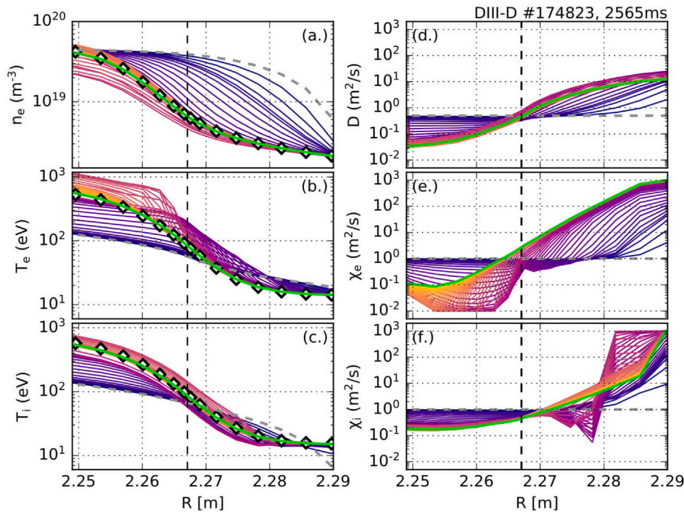
Fig. 5. Modeled outer mid-plane (a) n_e , (b) T_e and (c) T_i profiles are shown for a single time slice taken midway through the ELM cycle. Initial guesses are given as a gray dashed line, which then evolve via the autoUEDGE algorithm (blue through yellow) towards the final profile (green) based on comparison with data (white diamonds). Due to diagnostic constraints, the experimental OMP T_i profile is defined by assuming a constant T_i/T_e ratio in the edge region. Also shown is the evolution of the corresponding anomalous transport coefficients: (d) D , (e) \chi_e and (f) \chi_i . (For interpretation of the references to color in this figure legend, the reader is referred to the web version of this article.)
