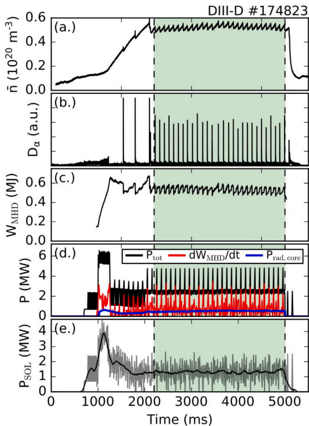
Fig. 2. Time traces for a low ELM frequency ( \sim 10 Hz) plasma discharge are shown. The line-averaged density (a), shows strong correlation with slow consistent ELMing behavior observable in the D_\alpha signal (b). The stored plasma energy ( W_{\text{MHD}} ) is shown in (c). The power radiated in the core P_{\text{rad,core}} and dW_{\text{MHD}}/dt are subtracted from the total injected power (d) to yield P_{\text{SOL}} - the power exiting the SOL (e). (For interpretation of the references to color in this figure legend, the reader is referred to the web version of this article.)
