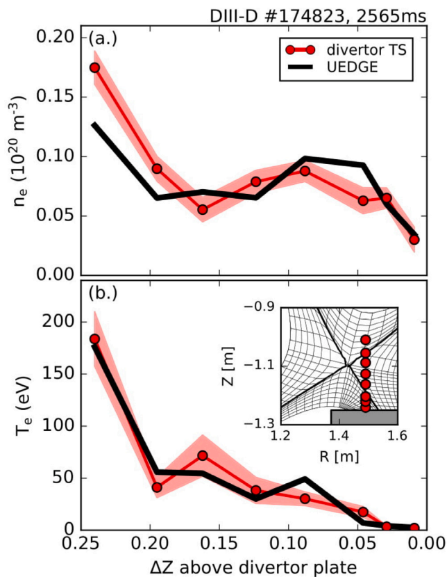
Fig. 6. Divertor Thomson measurements (red) of electron density (a) and temperature (b) are compared to synthetic diagnostics from UEDGE (black) for a single time slice mid-way through the ELM cycle, showing good agreement between modeling and experiment. (For interpretation of the references to color in this figure legend, the reader is referred to the web version of this article.)
